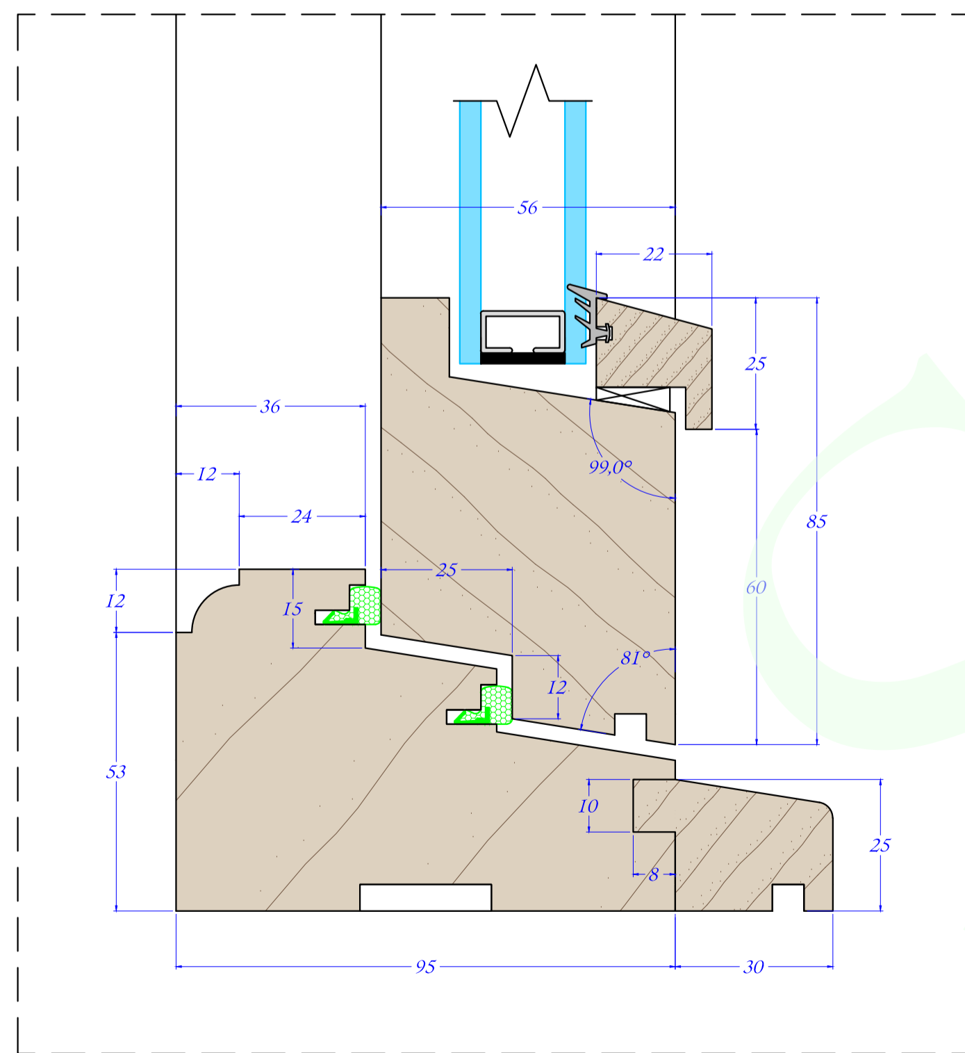
S03 SECTION DETAIL Scale: 1:1
