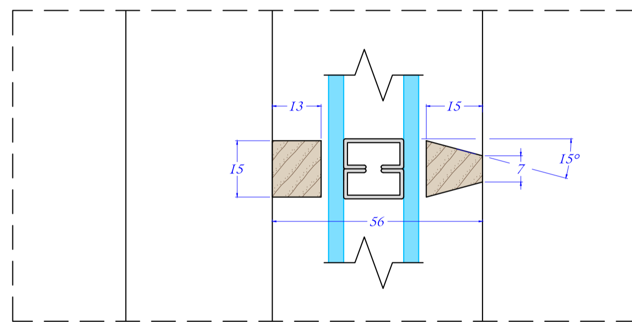
S02 SECTION DETAIL Scale: 1:1
