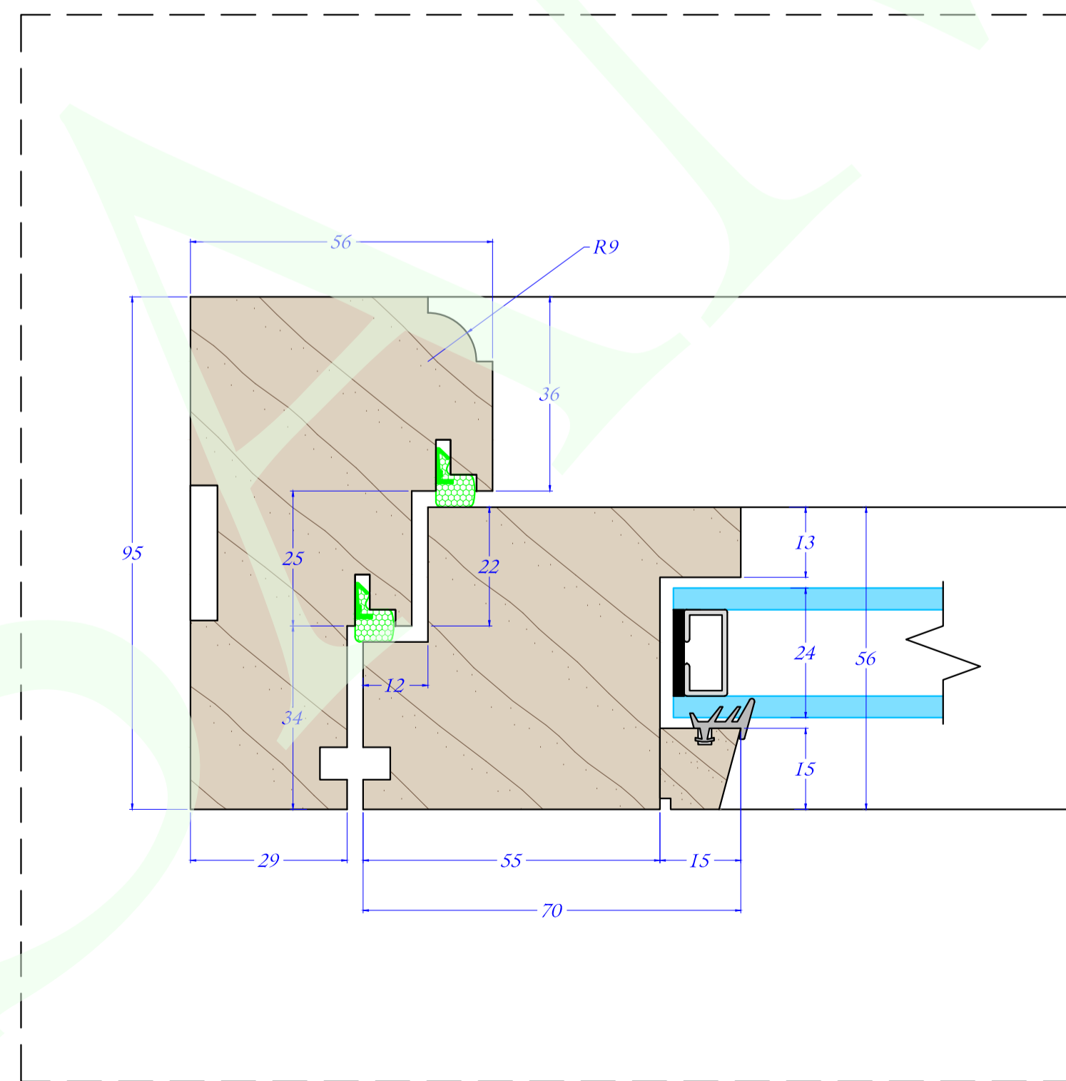
S04 SECTION DETAIL Scale: 1:1
