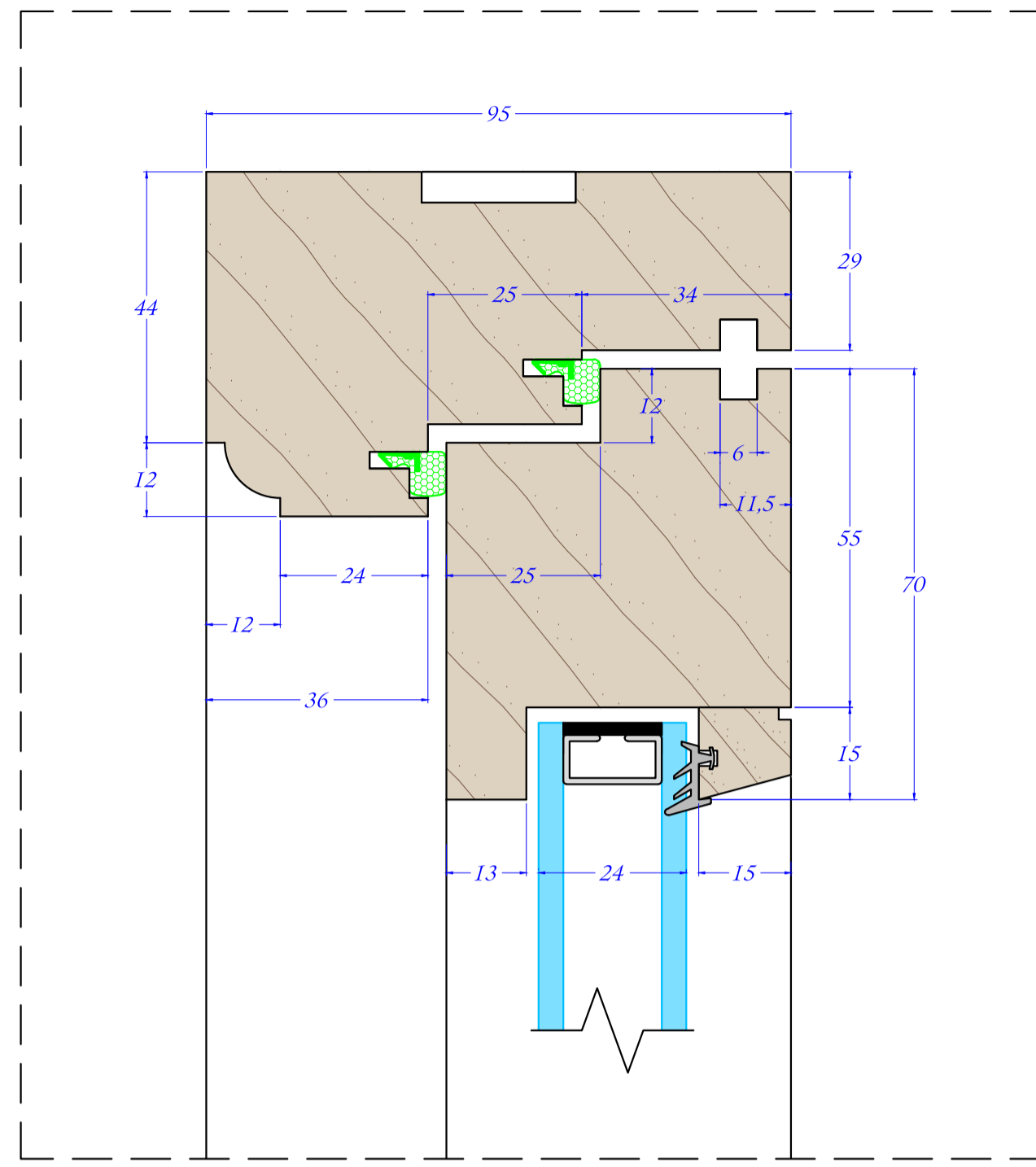
S01 SECTION DETAIL Scale: 1:1
